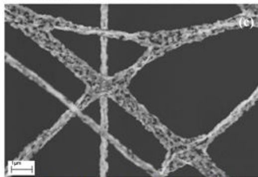
As-spun and oxidized mats
