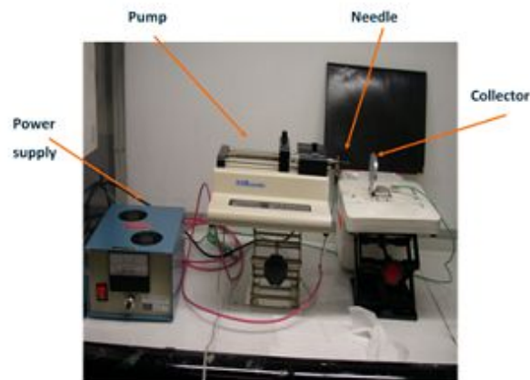
Electrospinning set up
